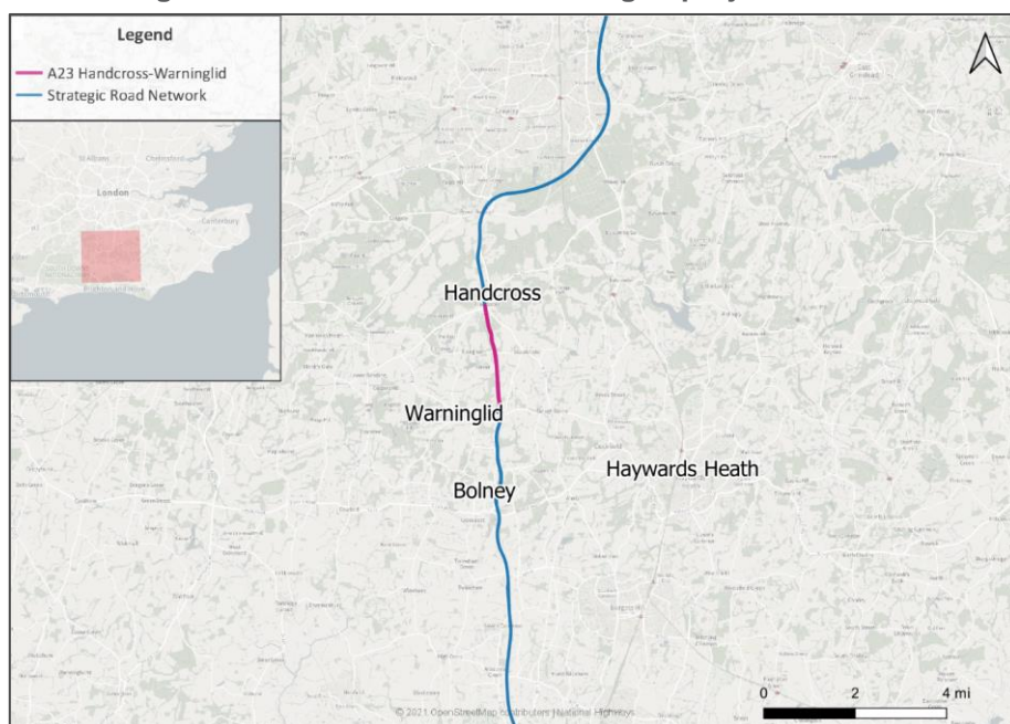
Figure 1: A23 Handcross to Warninglid project location
